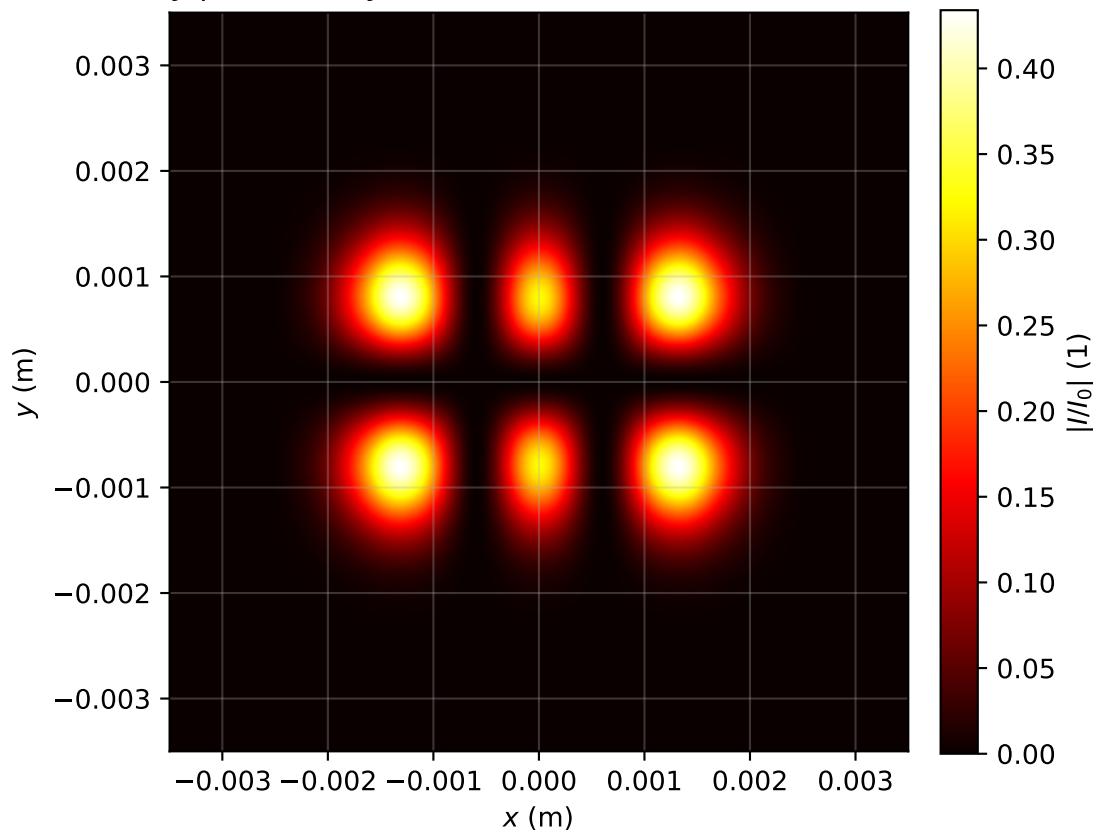
Intensity profile I(x, y, z = 2.627)/I_0 , P_{in}=1.0P_{cr} , artificial time
